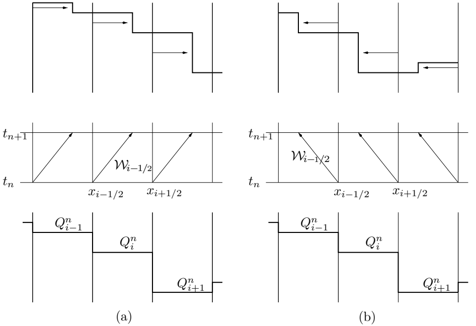
Fig. 4.5. Wave-propagation interpretation of the upwind method for advection. The bottom pair of graphs shows data at time t_n , represented as a piecewise constant function. Over time \Delta t this function shifts by a distance \bar{u} \Delta t as indicated in the middle pair of graphs. We view the discontinuity that originates at x_{i-1/2} as a wave \mathcal{W}_{i-1/2} . The top pair shows the piecewise constant function at the end of the time step after advecting. The new cell averages Q_i^{n+1} in each cell are then computed by averaging this function over each cell. (a) shows a case with \bar{u} > 0 , while (b) shows \bar{u} < 0 .
