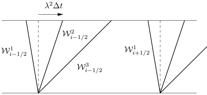
Fig. 4.7. An illustration of the process of Algorithm 4.1 for the case of a linear system of three equations. The Riemann problem is solved at each cell interface, and the wave structure is used to determine the exact solution time \Delta t later. The wave \mathcal{W}_{i-1/2}^2 , for example, has moved a distance \lambda^2 \Delta t into the cell.
